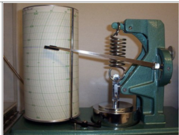
Abb. 4: Barograph
